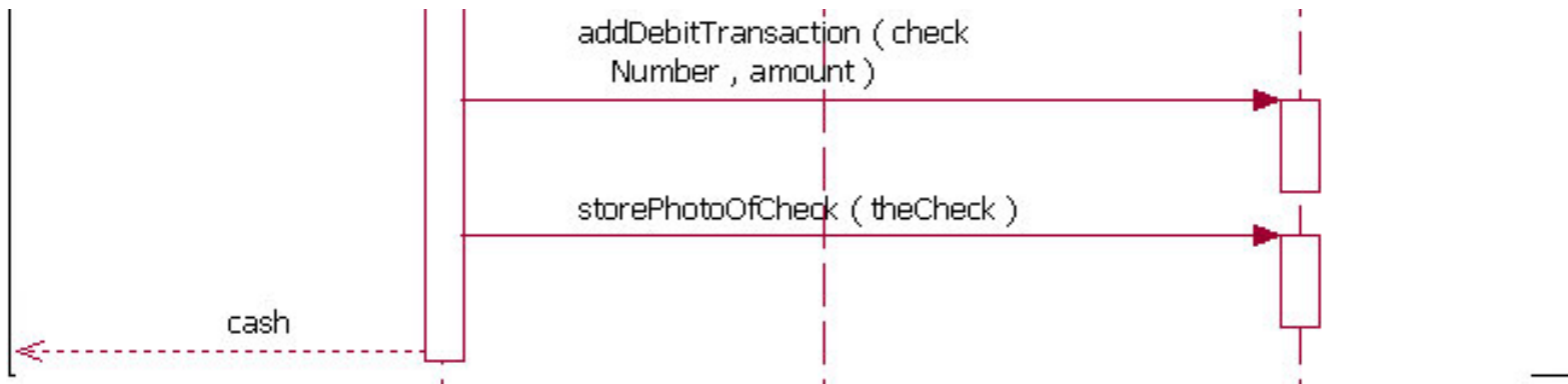
Figure 16: A reworking of the sequence diagram fragment from Figure 8, with the fragment using a break instead of an alternative
