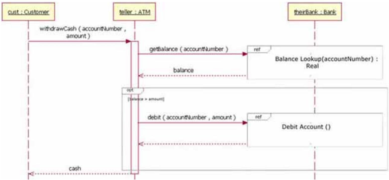
Figure 14: A reworking of Figure 11, using gates this time
