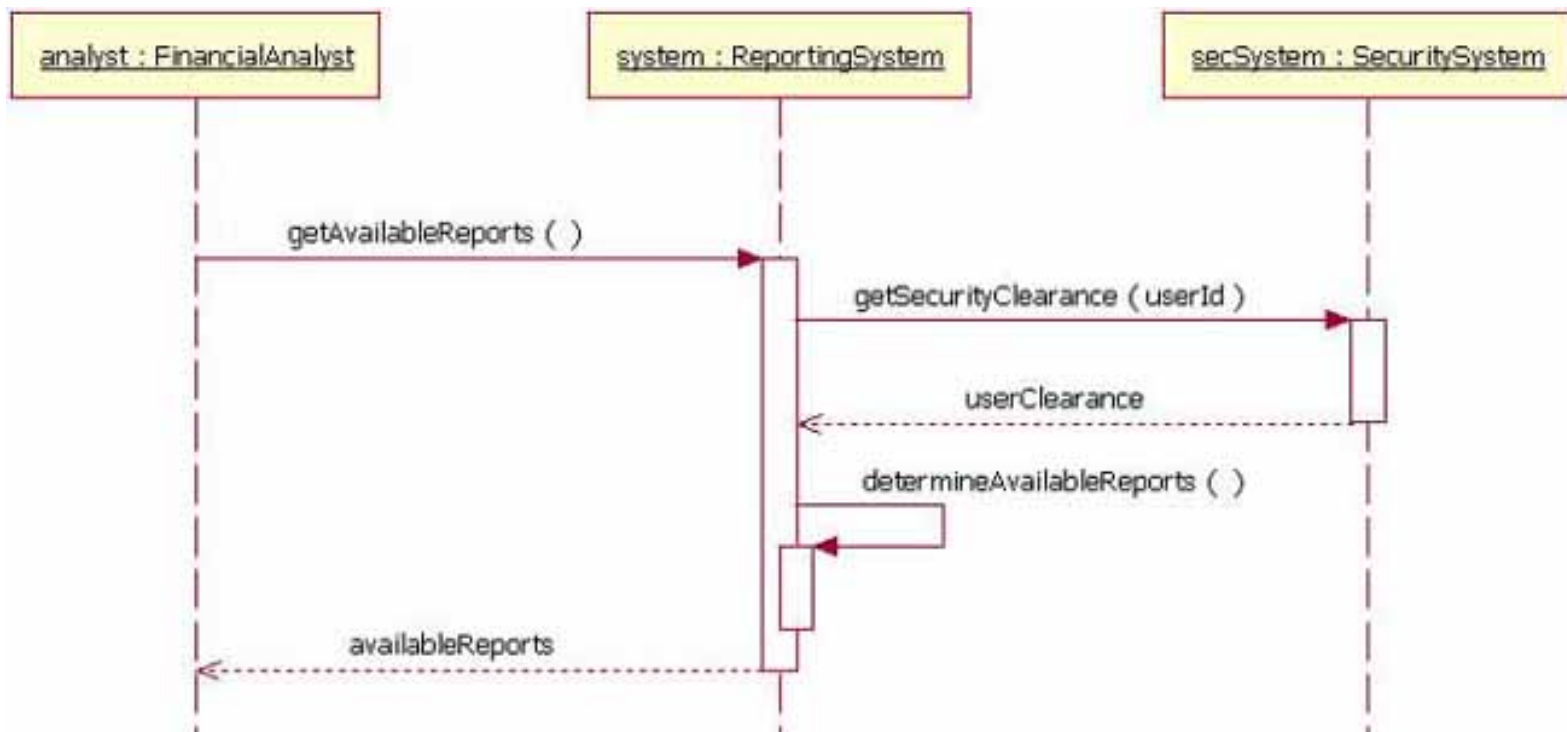
Figure 5: The system object calling its determineAvailableReports method
